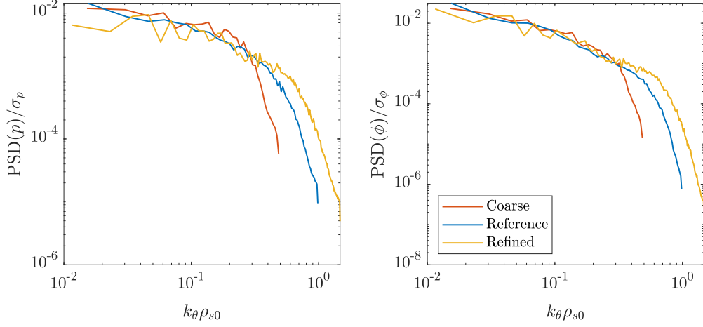
FIG. 15: Electron pressure p = nT (left panel) and electrostatic potential \phi (right panel) wavenumber spectra, normalized to the fluctuation levels, at the radial location R - R_{\text{LCFS}} = 2 cm for the “coarse” (red lines), “reference” (blue lines), and “refined” (yellow lines) simulations.
