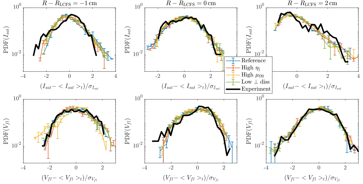
FIG. 7: PDFs of (I_{sat} - \langle I_{sat} \rangle_t) / \sigma_{I_{sat}} (first row) and (V_{fl} - \langle V_{fl} \rangle_t) / \sigma_{V_{fl}} (second row) at the three radial locations R - R_{LCFS} = -1 cm (first column), R - R_{LCFS} = 0 cm (second column), and R - R_{LCFS} = 2 cm (third column) for the experimental measurements (thick black lines) and the STORM simulations (thin color lines). The error bars represent one standard deviation of the results evaluated at \varphi = 0 and \varphi = \pi/4 .
