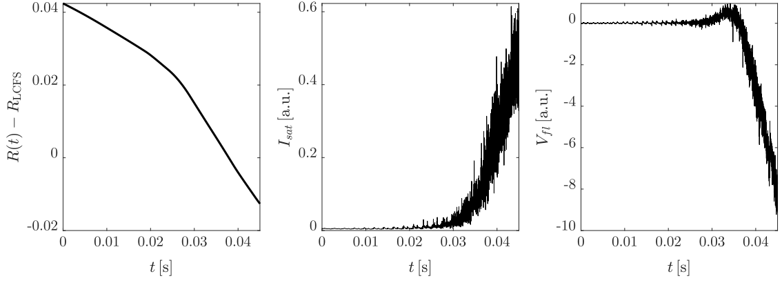
FIG. 16: Distance of the synthetic reciprocating probe from the LCFS (left panel) and synthetic time traces of ion saturation current (center panel) and floating potential (right panel) in arbitrary units.
