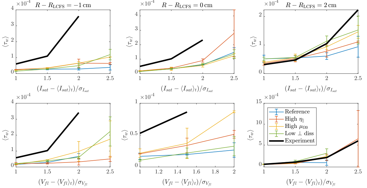
FIG. 12: Averaged waiting times between I_{sat} (first row) and V_{fl} (second row) maxima at the three radial locations R - R_{LCFS} = -1\text{ cm} (first column), R - R_{LCFS} = 0\text{ cm} (second column), and R - R_{LCFS} = 2\text{ cm} (third column) for the experimental measurements (thick black lines) and the STORM simulations (thin color lines). The error bars represent one standard deviation of the results evaluated at \varphi = 0 and \varphi = \pi/4 .
